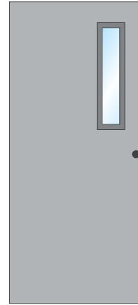
HOLLOW METAL NARROW LITE 6" X 27" LITE
